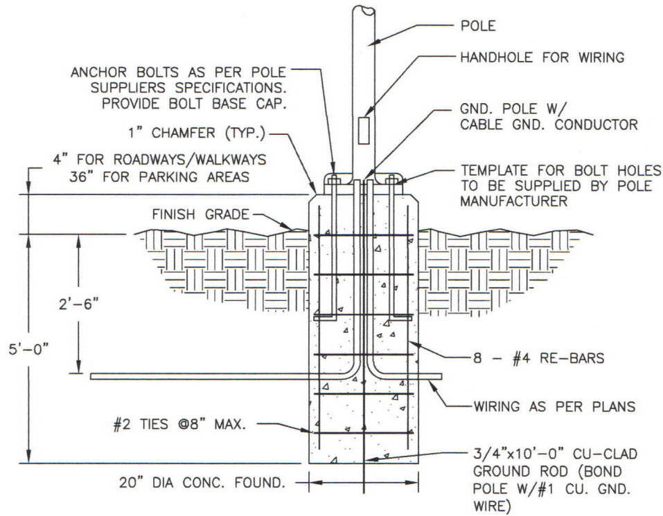
20" LIGHT POLE FOUNDATION FOR MAXIMUM 20' POLE HEIGHT N.T.S.
